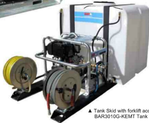
▲ Truck mount with roll frame
